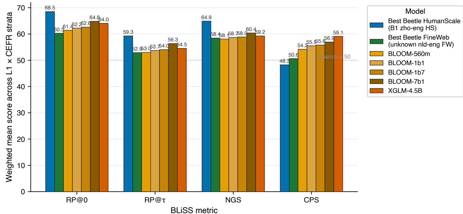
Best Beetle models vs LLM baselines on BLiSS (final checkpoint)
